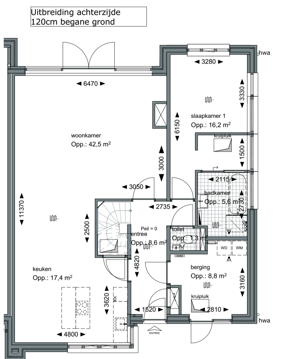
1:100 00 Begane grond
