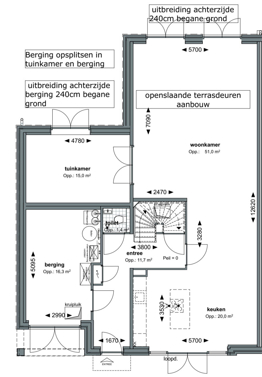
1:100 00 Begane grond
