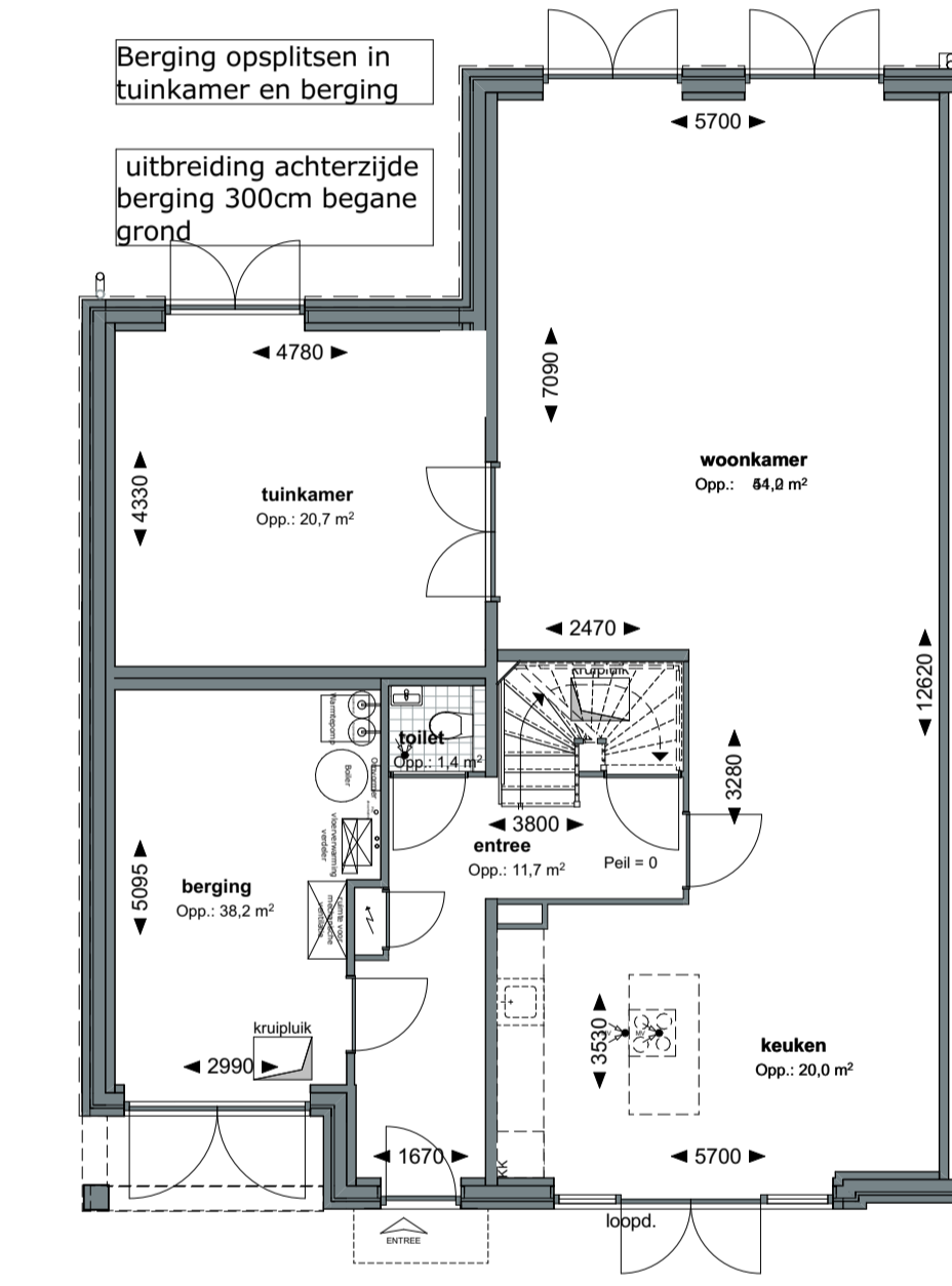
1:100 00 Begane grond
