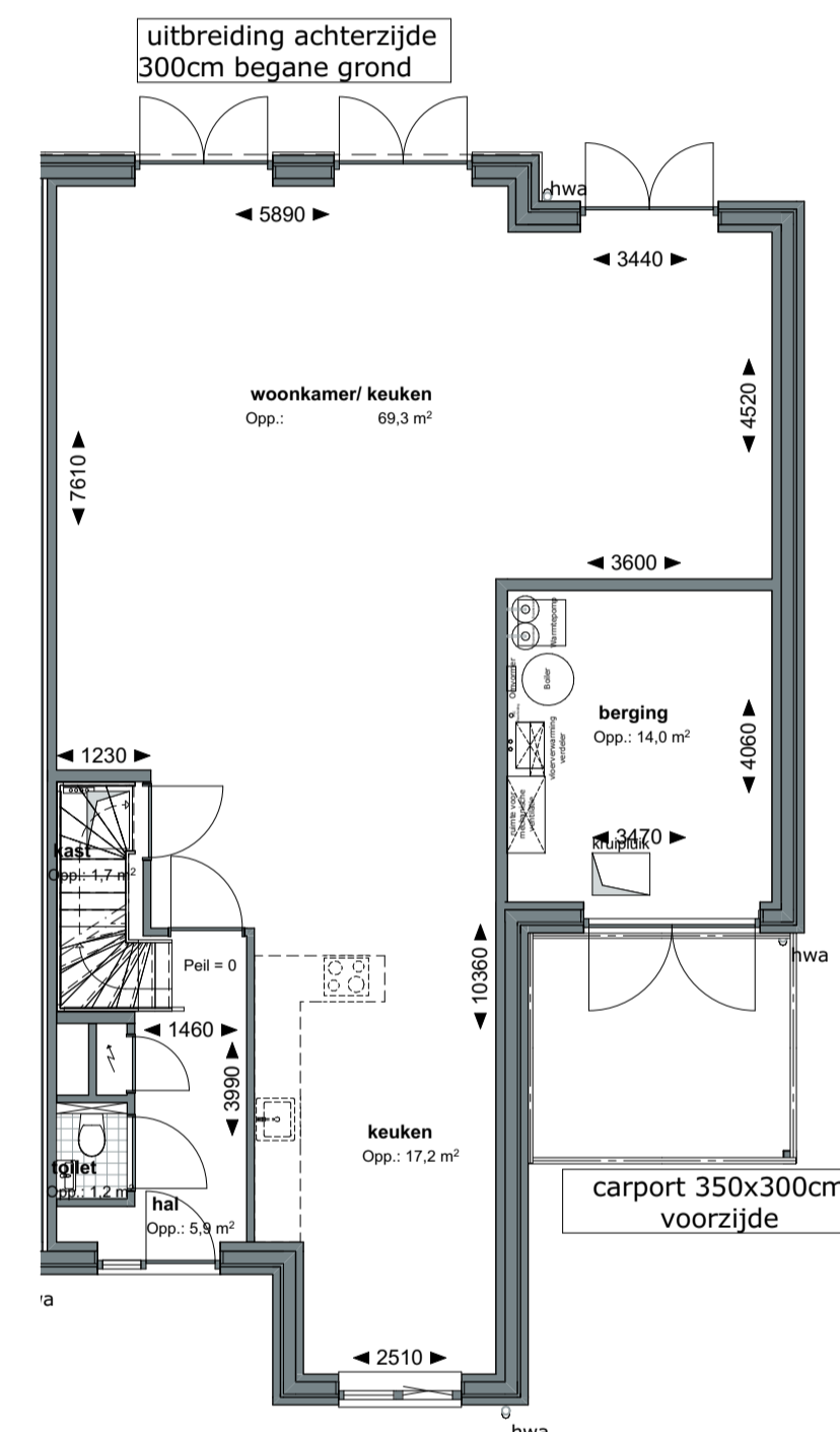
1:100 00 Begane grond
