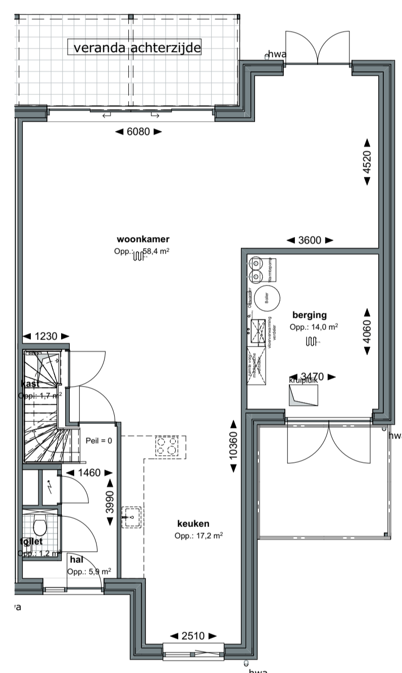
1:100 Begane grond veranda
