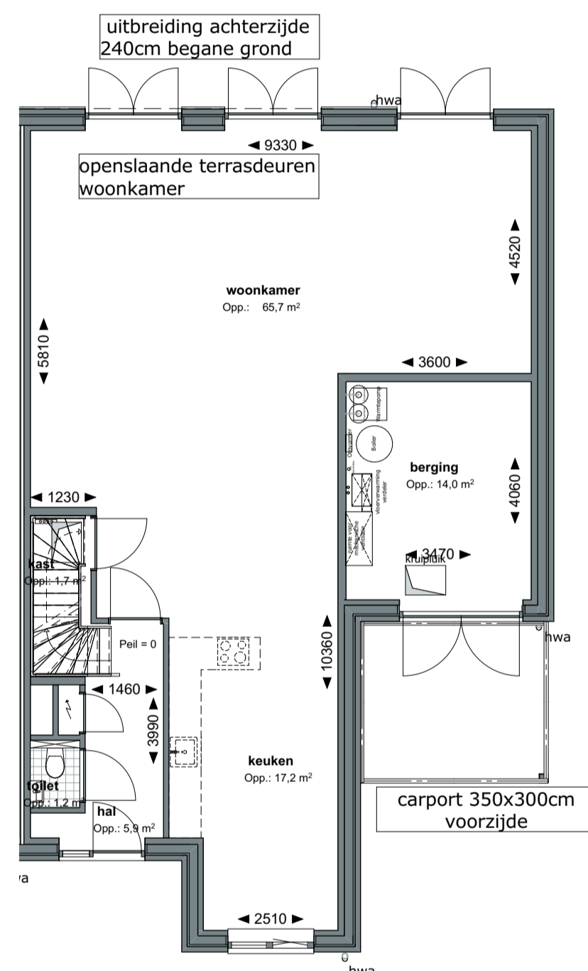
1:100 00 Begane grond
